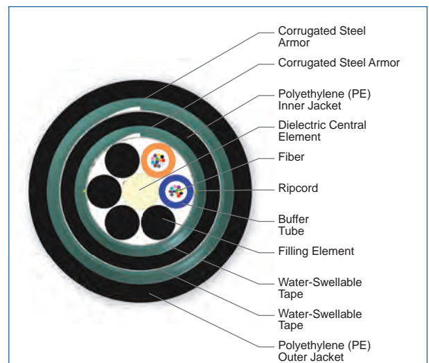
Cross Section of Part Number: 024EUD-T4101D20
